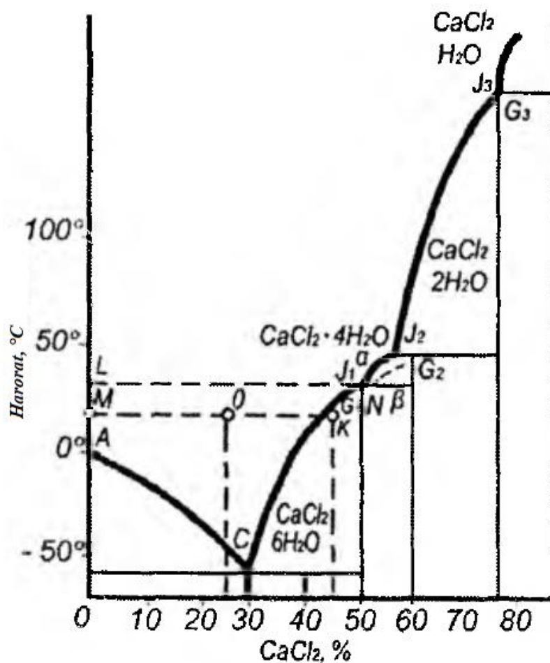
6.3-rasm. \text{CaCl}_2 \cdot \text{H}_2\text{O} sistemaning eruvchanlik diagrammasi.
