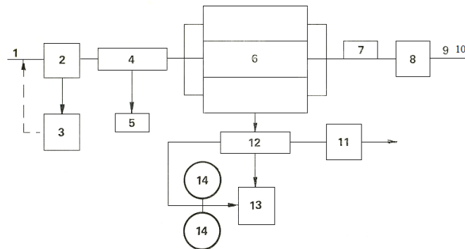
3.10-rasm. Oqava suvlarning mexaniq tozalash sxemasi
