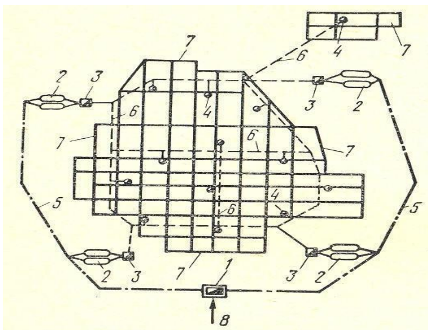
4.10-rasm. SHaharning gaz bilan ta'minlanish uch pog'onali sxemasi:
