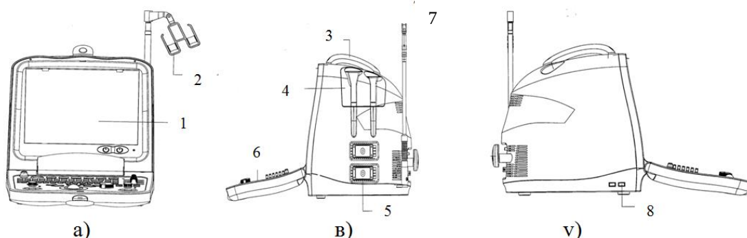
2.37 – Rasm. UT qurilmasi monitorining a – yuz, b – chap yon va v – o'ng yon tomonlardan ko'rinishi: 1 – monitor ekran, 2 - datchik kabeli uchun ilgak, 3 – monitorni tashish uchun ruchka, 4 – datchikni ushlab turuvchi joy, 5 - datchikning raz'yomi, 6 - boshqaruv pulti, 7 - tashqi stoyka, 8 - YuSB port
