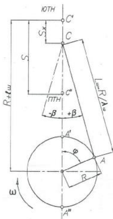
3-rasm. Markaziy krivoship-shatun mexanizmning sxemasi
