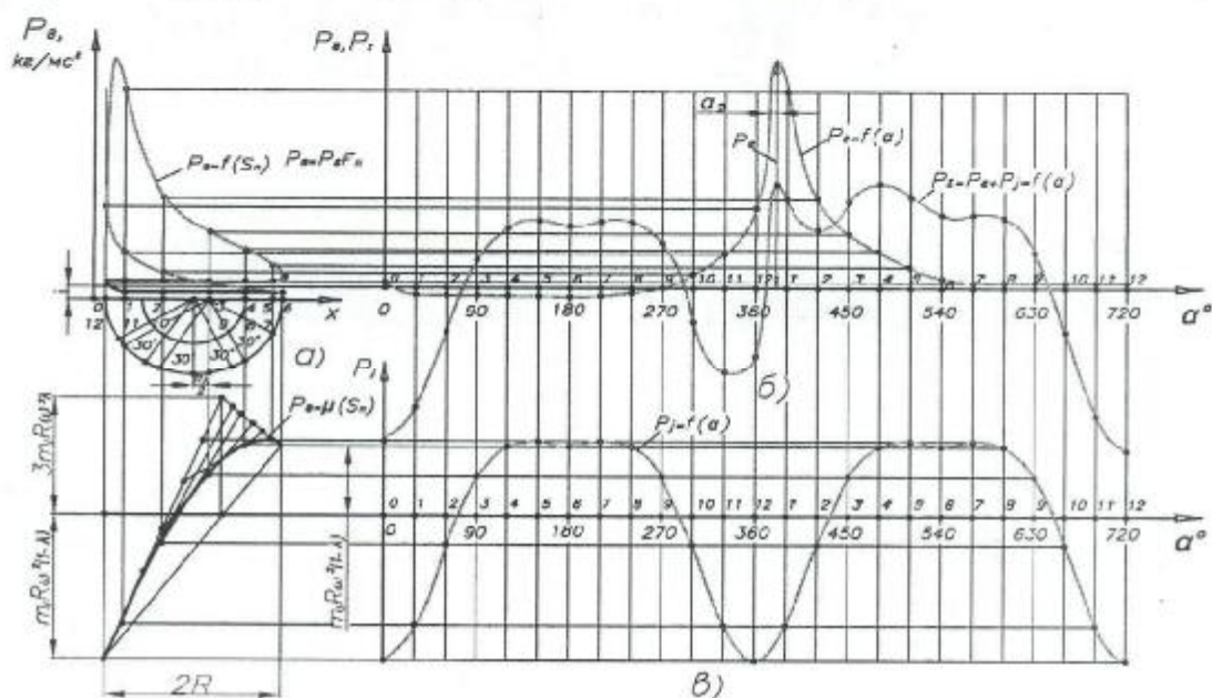
7-rasm. To'rt taktli dvigatelning P_r , P_f , va P_z kuchlarini tuzish
