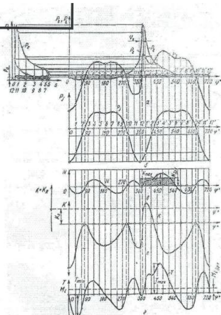
8- rasm. Krivoship-shatun mexanizmidagi kuchlarning tirsakli val burilish burchagi bo'yicha o'zgarish grafigi
