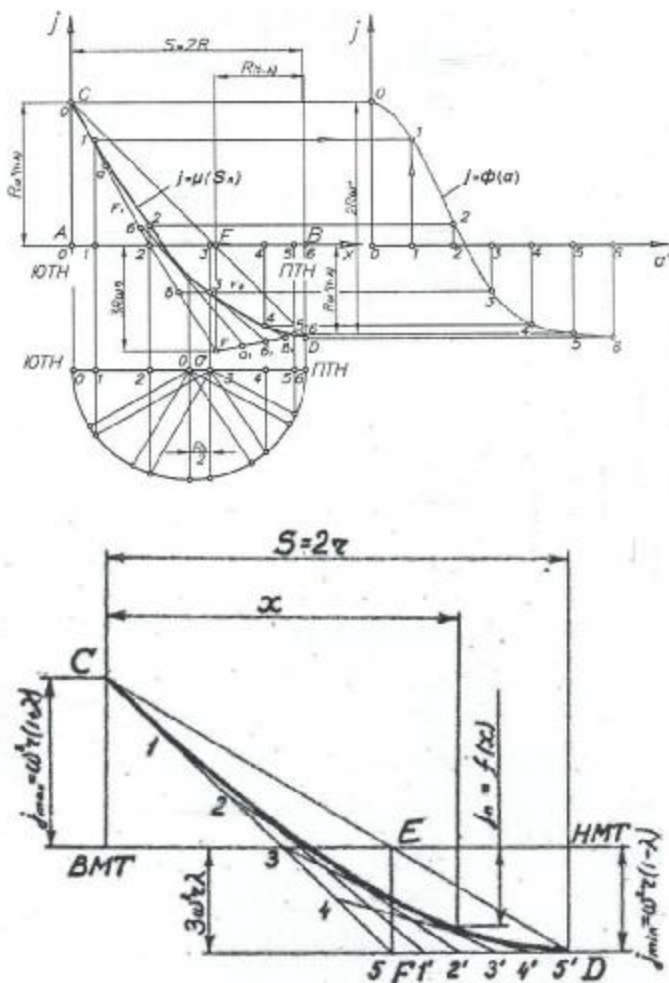
5-rasm. Urunma usuli bilan porshenning tezlanish egri chizig'ini qurish grafigi
