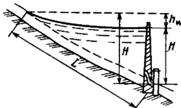
41-rasm. GES bosimni vujudga keltirishning to'g'ri usuli
