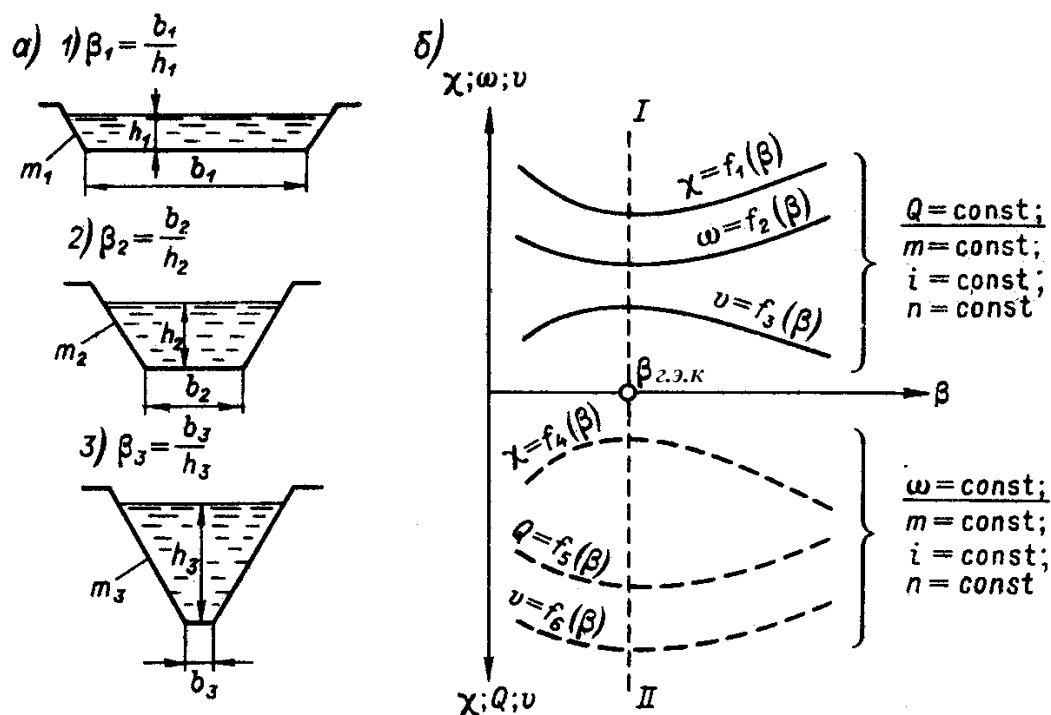
35-rasm. Trapetsiadal kanalning \beta nisbiy kengligining o'zgarishi natijasida \chi , \omega , v , Q tirik kesim elementlarining o'zgarishi
