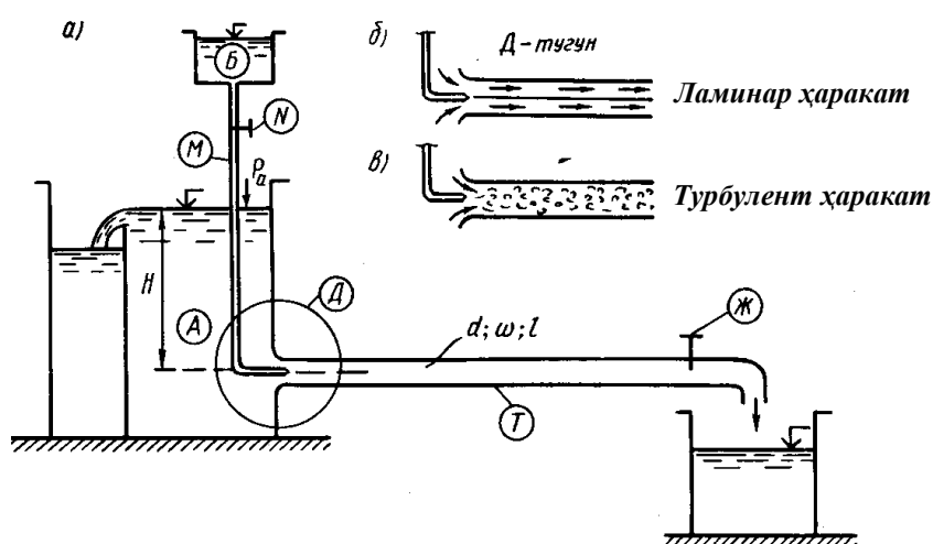
14-rasm. Reynolds qurilmasining sxemasi
