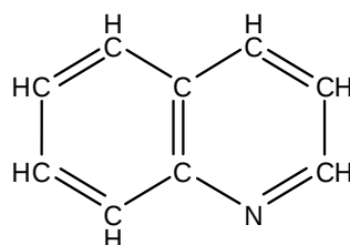
xinolin
