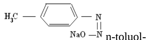
Benzol-antidiazogidrat
