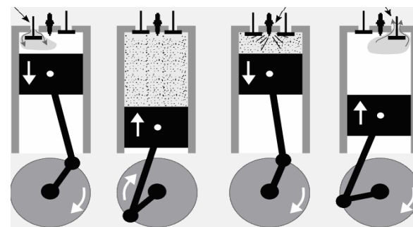
2.8-rasm. Karbyuratorli dvigatelda yonish jarayoni.
