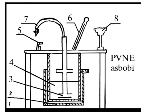
5.7-rasm. Moylarning alanganish haroratini yopiq tigelda aniqlash asbobi.
