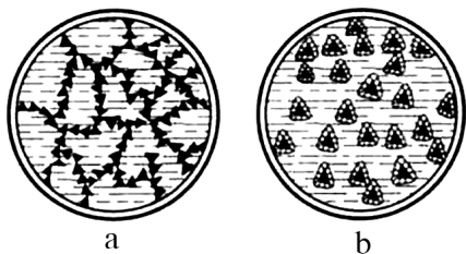
5.3-rasm. Past haroratdagi moylarda kristal to'ra hosil bo'lishi: a-qo'shilmasiz moy, b-qo'shilmali moy
