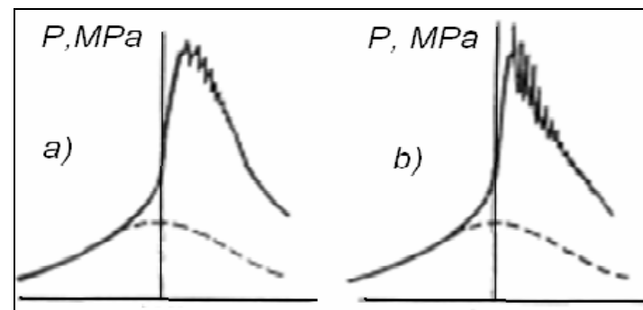
2.11-rasm. Detonatsiyali yonish jarayonining indikator diagrammasi: Kuchsiz (a) va kuchli (b) detonatsiyali yonish diagrammalari.
