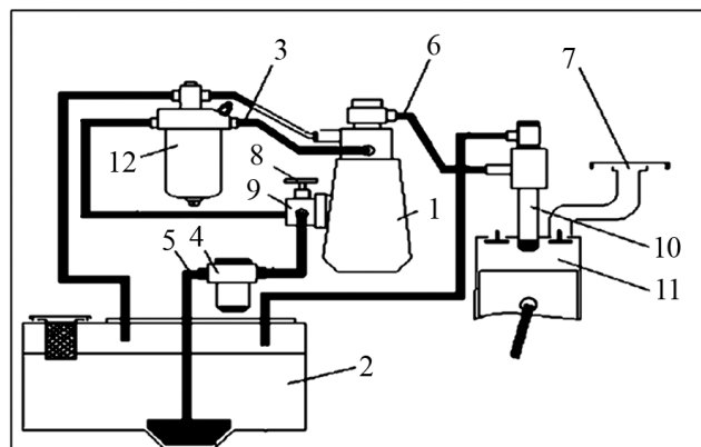
3.7-rasm. Dizel dvigatelining ta'minlash tizimi: 1- yonilg'i nasosi, 2- yonilg'i baki, 3,5,6- truboprovod, 4- dag'al tozalash filtri, 7- havo tozalagich, 8-ventil, 9-haydash nasosi, 10-forsunka, 11- yonish kamerasi, 12- mayin tozalash filtri
