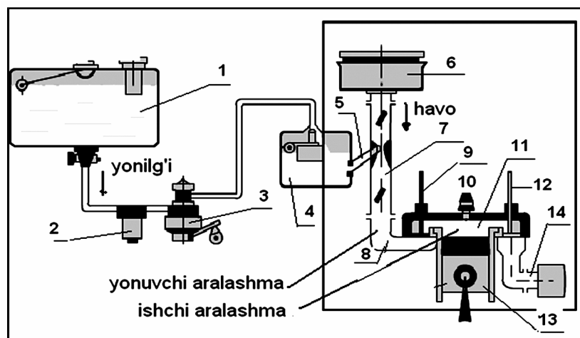
2.7 -rasm. Karbyurator dvigatelining ta'minlash shemasi:
