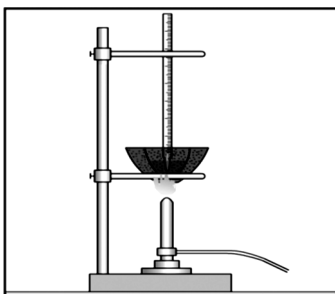
5.6- rasm. Moylarning alanganish haroratini ochiq tigelda aniqlash asbobi.
