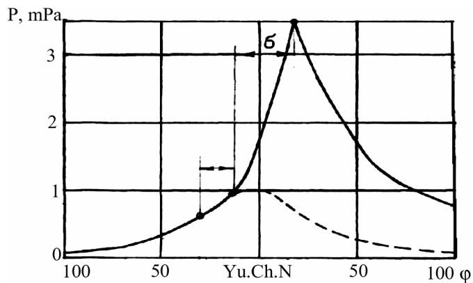
2.10-rasm. Uchqun bilan alangalanadigan dvigatellarning indikator diagrammasi.
