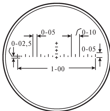
58-rasm. Durbinning burchak o'lchash turi.
