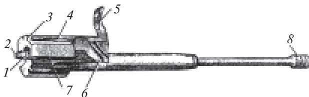
86-rasm. Zatvor ramasi, gaz porsheni bilan birgalikda:
