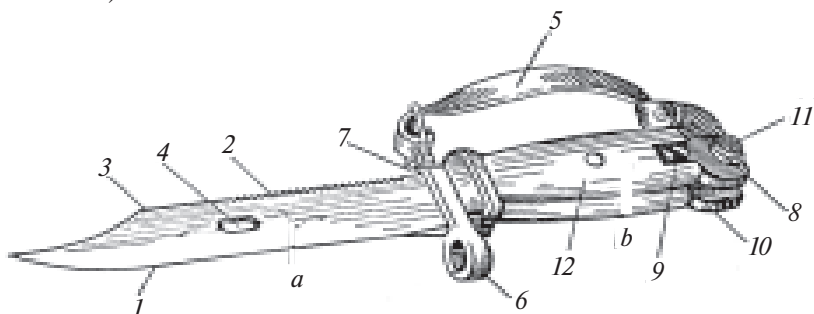
93-rasm. Nayza-pichoq:
