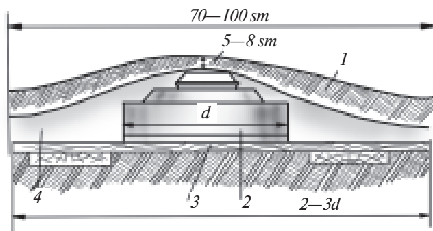
69-rasm. Tankka qarshi minaning yumshoq (zax) yerda o'rnatilishi:
