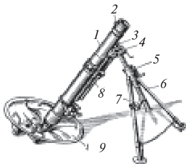
34-rasm. 120 mm.li minomyot:
