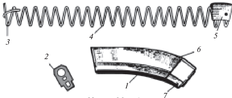
92-rasm. Magazin:
