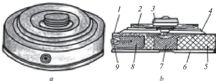
64-rasm. Tankka qarshi TM-57 mina MVZ-57 portlagich bilan birga ko'rinishi:
