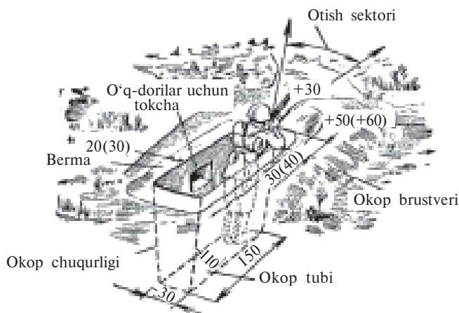
38-rasm. Avtomatdan turib otish uchun okop.
