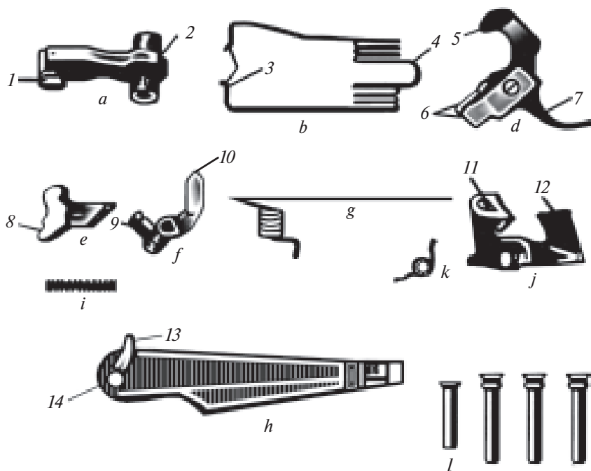
90-rasm. Zarbdor-tepki mexanizmining qismlari:
