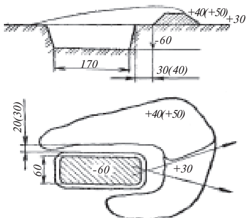
37-rasm. Avtomatdan tizzalab otish uchun okop.
