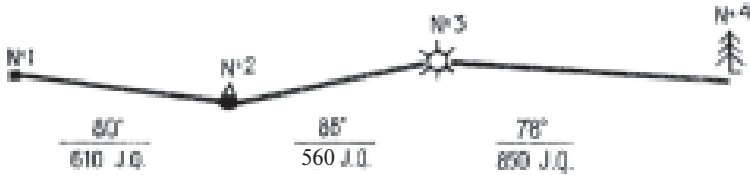
77-rasm. Azimutlar bo‘ylab qadamlab yurish chizmasi ( j.q. — juft qadam).
