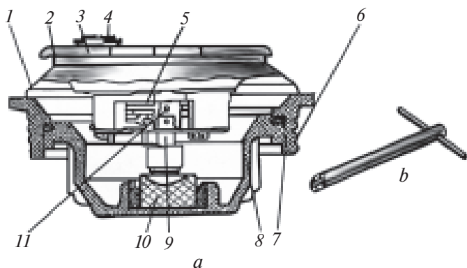
68-rasm. MVCH-62 portlatgich:
