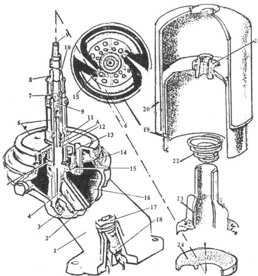
4.9-rasm. Dvigatelning markazdan qochma moy tozalagichi:
