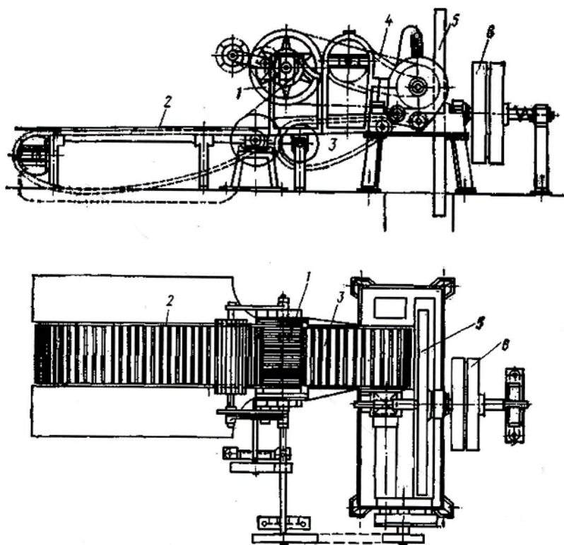
3.4-rasm. Diskli somon maydalash dastgohi:
