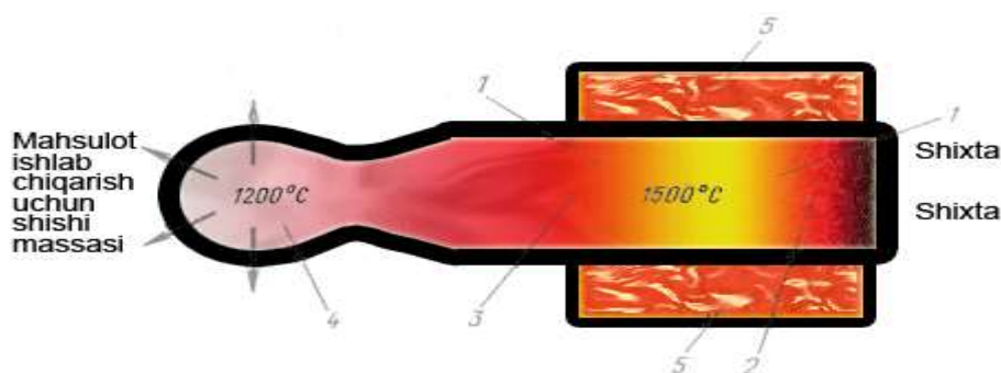
84rasm. Vannasimon shisha pishirish sxemasi.
