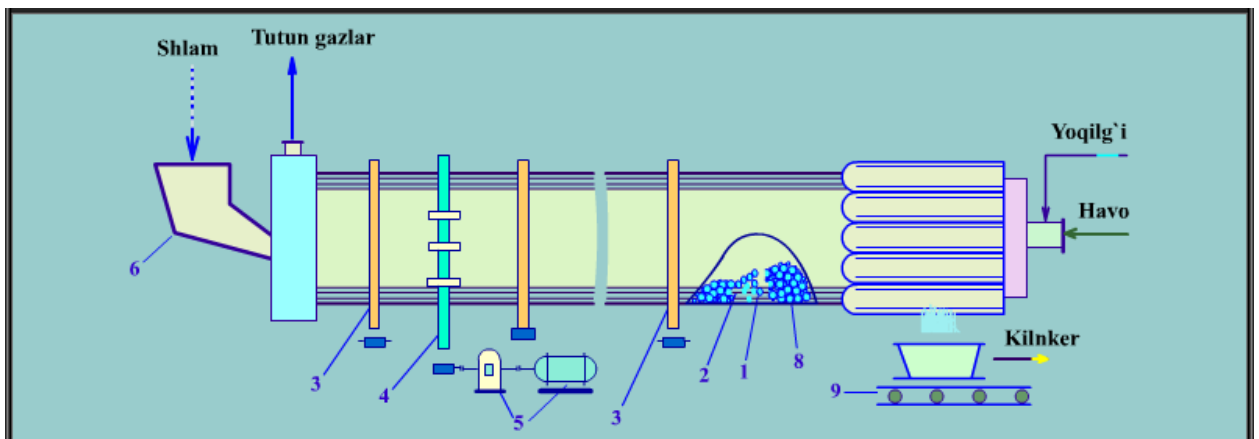
83-rasm. Sement klinkeri ishlab chiqarish uchun aylanuvchi barabanli pech.
