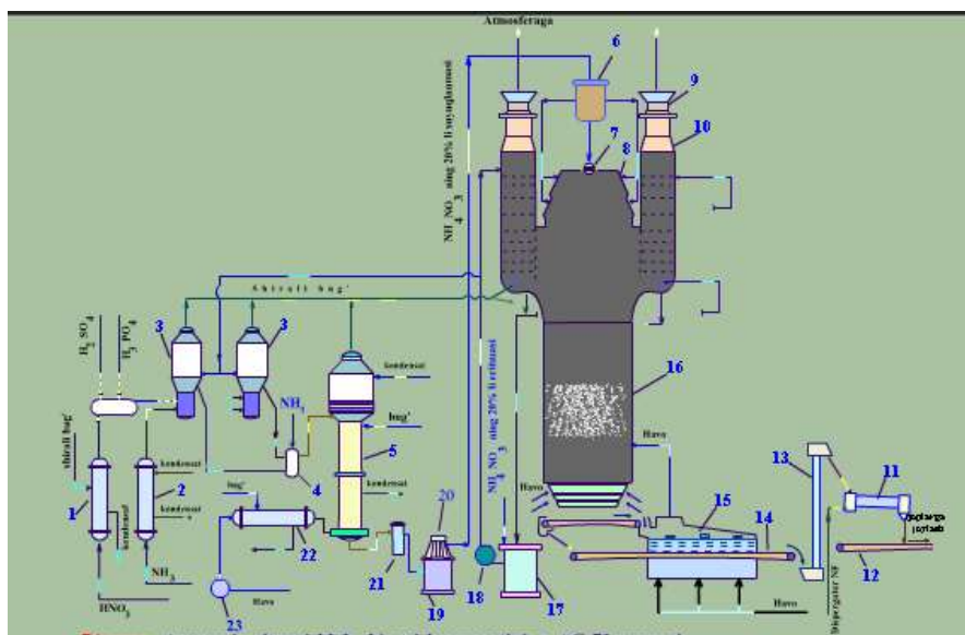
73-rasm. Ammoniy nitrat ishlab chiqarish agregatining AC-72 sxemasi.
