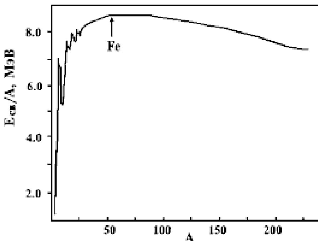
Rasm 3. Solishtirma bog'lanish energiyasi E_{bog}/A – ning massalar soni A – ga bog'lanishi.
