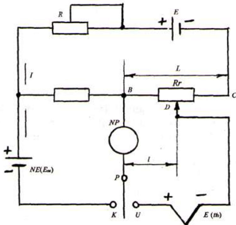
35 – rasm. Potensiometrning prinsipial sxemasi.
