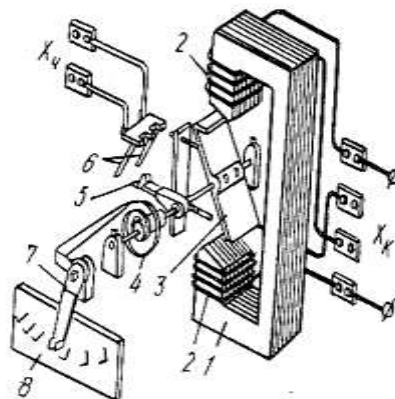
85-rasm. Maksimal tok releli:
