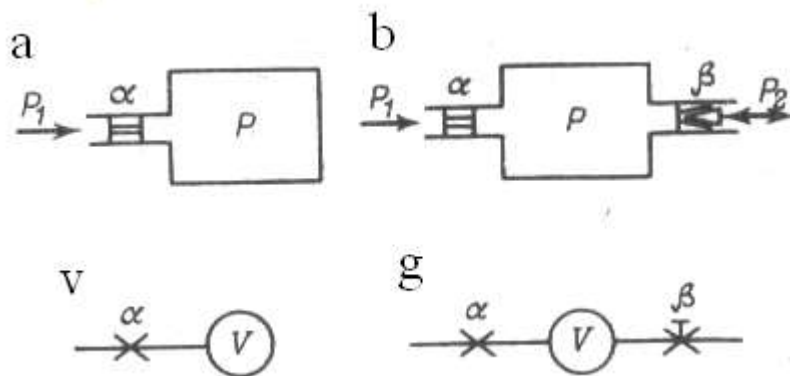
89- rasm. Pnevmokameraning sxemasi
