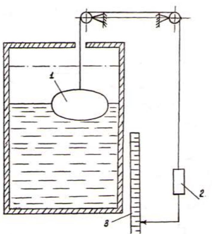
45-rasm. Qalqovichli sath o'lchagich.
