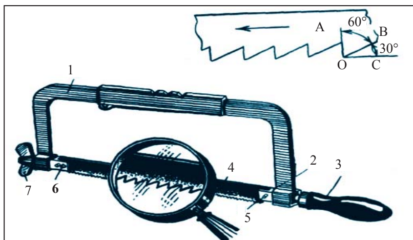
8-su'wret. Tutqali' slesarli'q pi'shqi'si': 1-tiykar (ramka); 2-quyri'q; 3-tutqa; 4-pi'shqi' polotnosi'; 5-shtift; 6-tarti'wshi' vint; 7-qulaqli' gayka.
