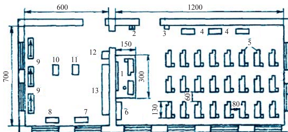
30-su'wret. Ag'ash ustashi'li'g'i' woqi'w ustaxanasi'nda jumi's wori'nlari'ni'n' shamalap jaylasi'w rejesi: 1 – mug'allimnin' jumi's worni'; 2 – qol juwi'w quri'lmasi'; 3 – aptechka; 4 – a'sbap-u'skene ha'm meteriallar stellaji'; 5 – stanoklar; 6 – woqi'w-ko'rgizbe qurallar stellaji'; 7, 8, 9, 10, 11 – frezalaw, burg'i'law, ag'ashti' islew tokarli'q stanoklari', joni'w, pi'shqi'law stanoklari'; 12 – shar; 13 - materiallar tekshesi.
