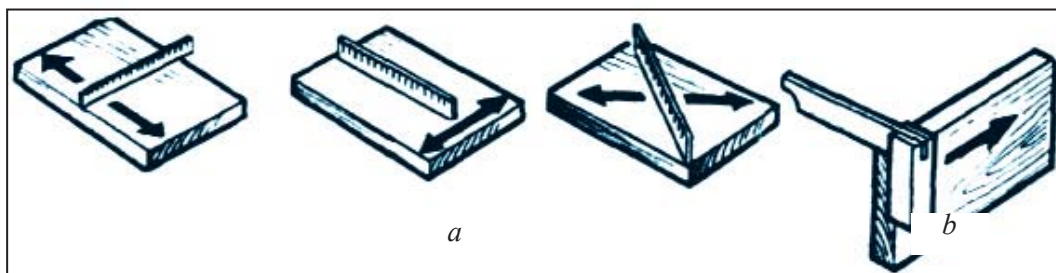
54-su'wret. Betlerdin' tegisligin si'zg'i'sh (a) yaki genuya (b) da tekseriw.
