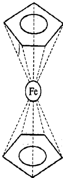
35-rasm. Ferrosen molekulasining tuzilishi.
