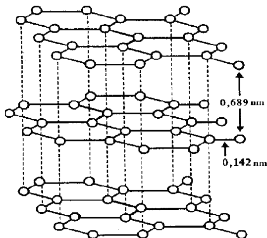
39-rasm. Grafit kristall panjarasining tuzilishi.
