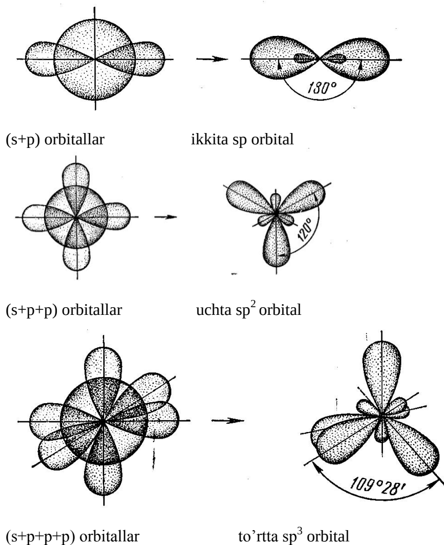
19-rasm. Valent orbitallarining gibridlanishi.
