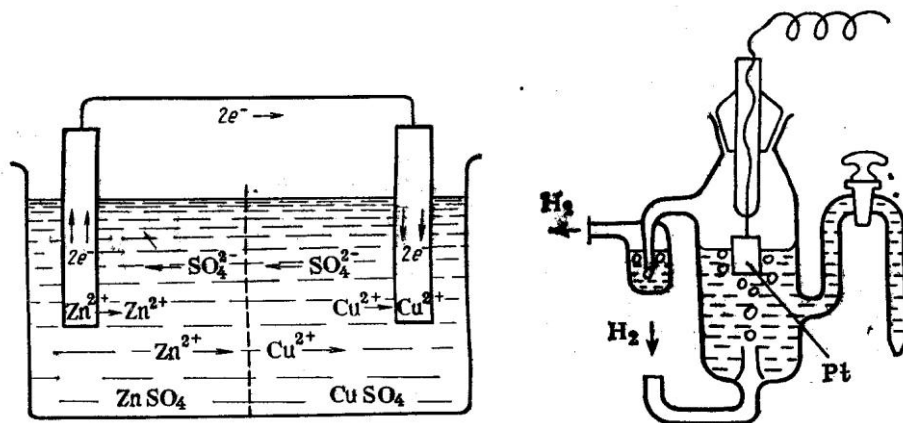
28-rasm. Mis va ruxdan iborat galvanik zanjirda ionlarning harakatlanishi.
