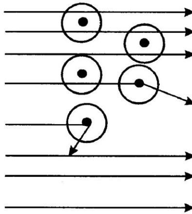
6-rasm . \alpha - zarrachalarning metall dan o'tishida og'ishi.
