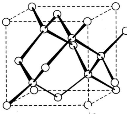
38-rasm. Olmos kristall panjarasining tuzilishi.
