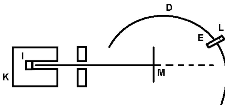
5- rasm. \alpha - zarrachalarning yupqa metal pardadan o'tishi.
