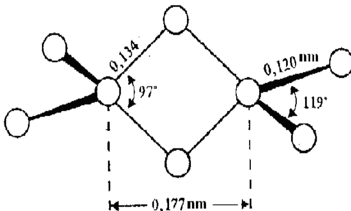
37-rasm. Boretan molekulasi tuzilishi
