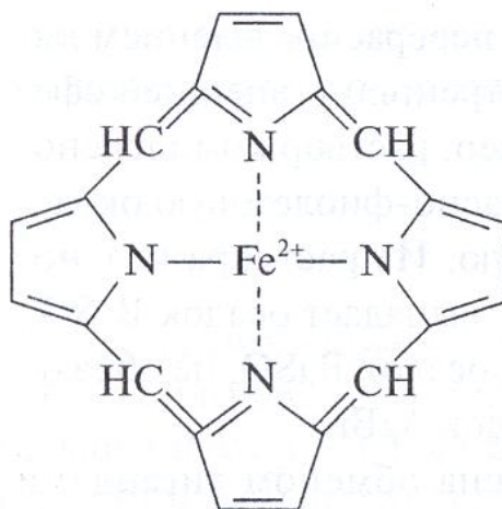
36-rasm. Gemoglobinning tuzilishi.
