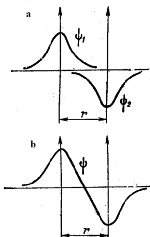
21-rasm. 1s- atom orbitallardan bo'shashtiruvchi orbitallarning hosil bo'lishi.
