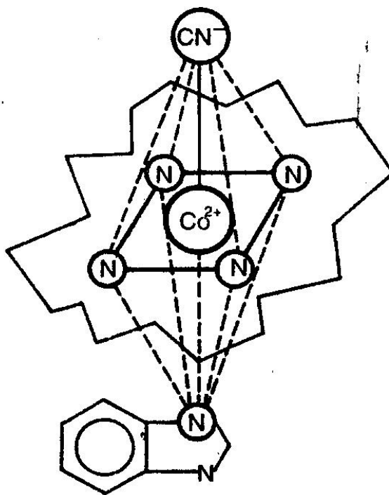
26-rasm. Vitamin \text{B}_{12} yoki siankobalamin molekulasi tuzilishi.
