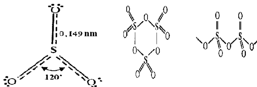
47-rasm. SO 3 molekulari monomer, dimer va trimer holatidagi tuzilishi.
