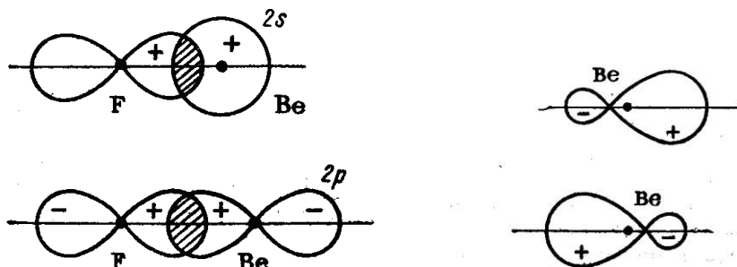
17-rasm. \text{BeF}_2 molekulasini hosil bo'lishida 2s- va 2p-orbitallarining qoplashi.
