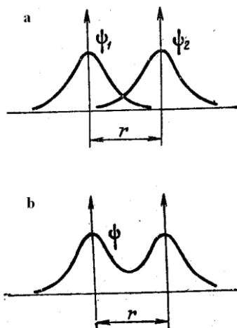
20-rasm. 1s-atom orbitallardan bog'lovchi orbitallarning hosil bo'lishi.
