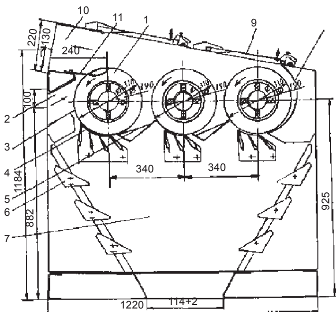
1.18-rasm. 2VP rusumli tola tozalagich:
