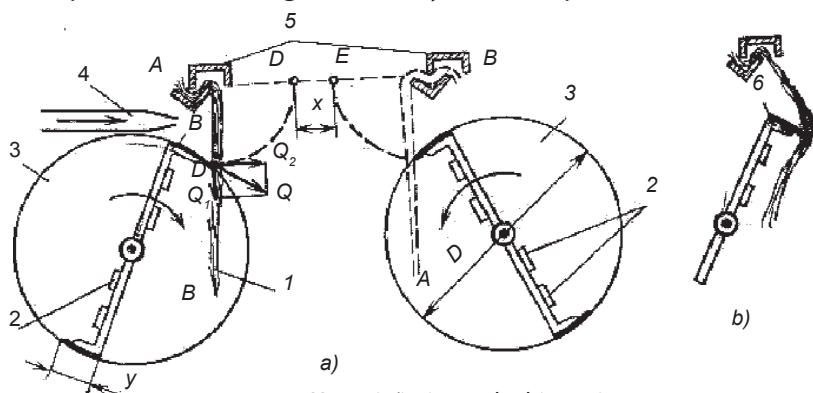
4.6-rasm. Xom zig'irni savash chizmasi:
