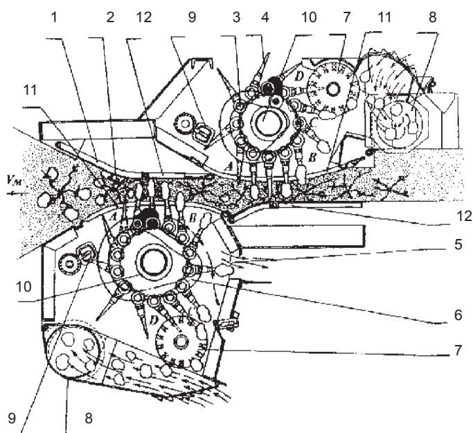
1.6-rasm. Gorizontall shpindelli paxta terish apparatining texnologik ish jarayoni:
