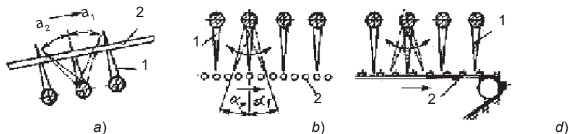
4.7-rasm. Chiqindilarni silkitish va savash mashinasining chizmasi:
