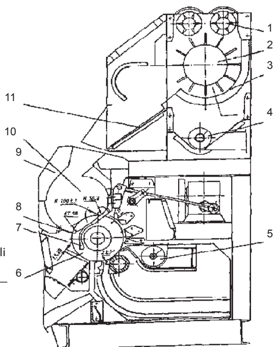
1.14-rasm. 5DP-130 arrali jin:
