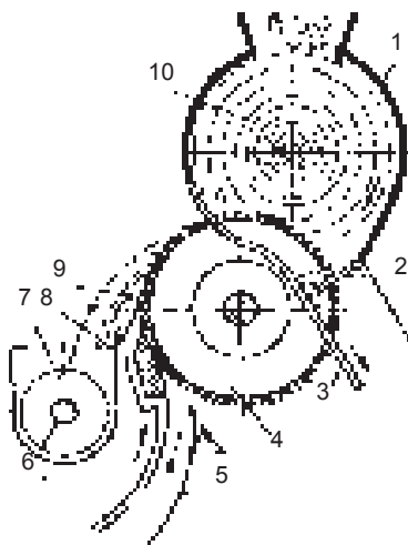
1.15-rasm. Arraning chigitli paxta valigiga ta'siri chizmasi:
