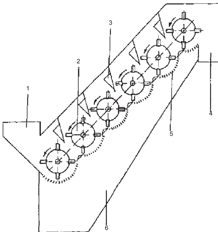
1.21-rasm. ON—6—3 rusumli tola tozalagichi:
