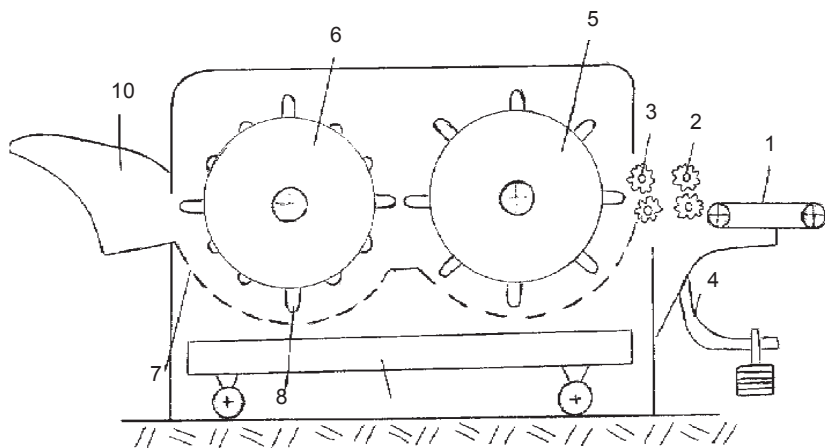
5.2-rasm. Junni titish mashinasi:
