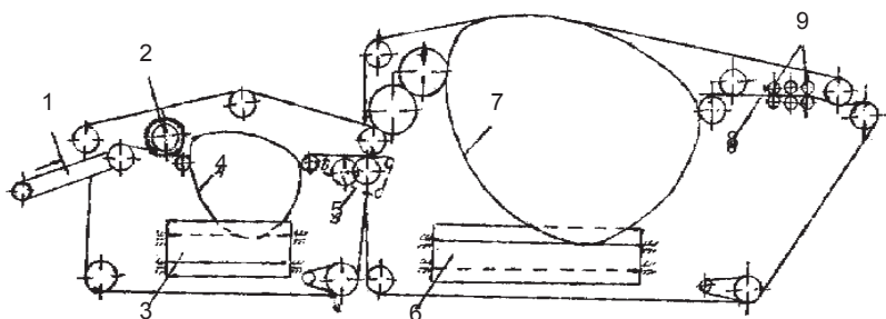
3.10-rasm. ALT rusumli titish-yuvish mashinasining texnologik chizmasi:
