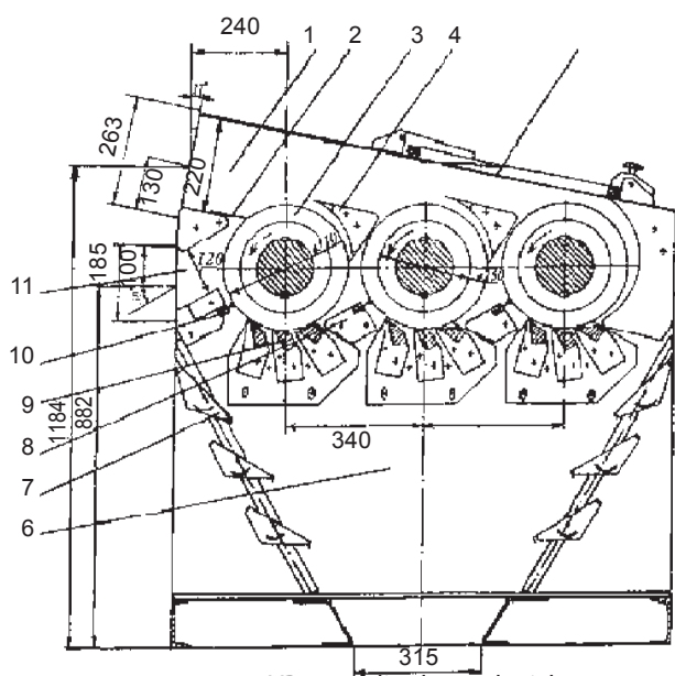
1.17-rasm. 1VP rusumli tola tozalagich:
