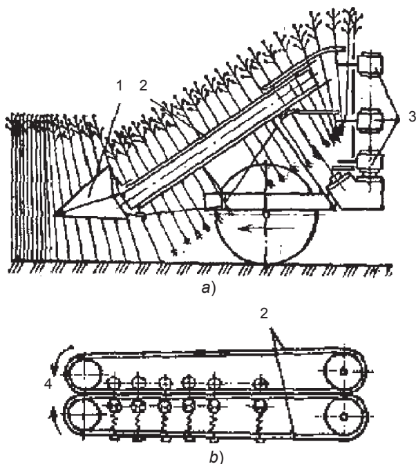
4.2-rasm. Zig'irpoyani yanchish mashinasining chizmasi:
