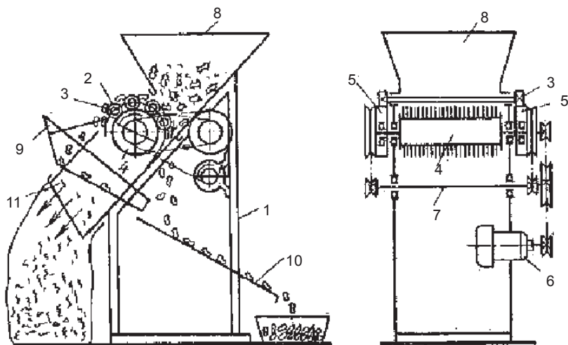
2.8-rasm. Pillani saralash va tozalash mashinasi:
