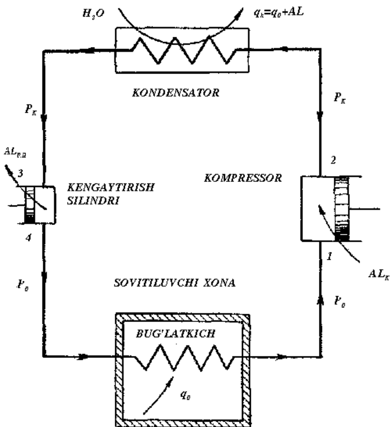
3-rasm. Sovitish mashinasining sxemasi
