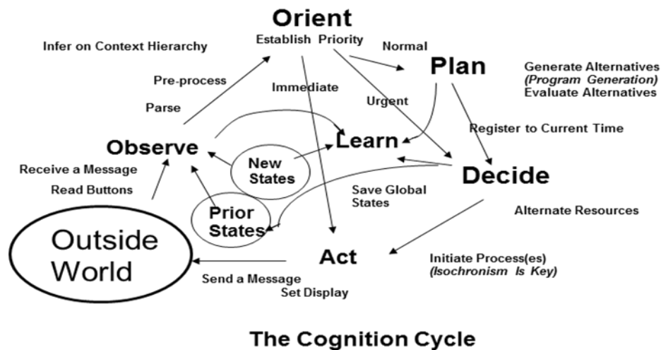
Figure 9 - Observe, orient, plan, learn, decide and act, OODA mechanism.
