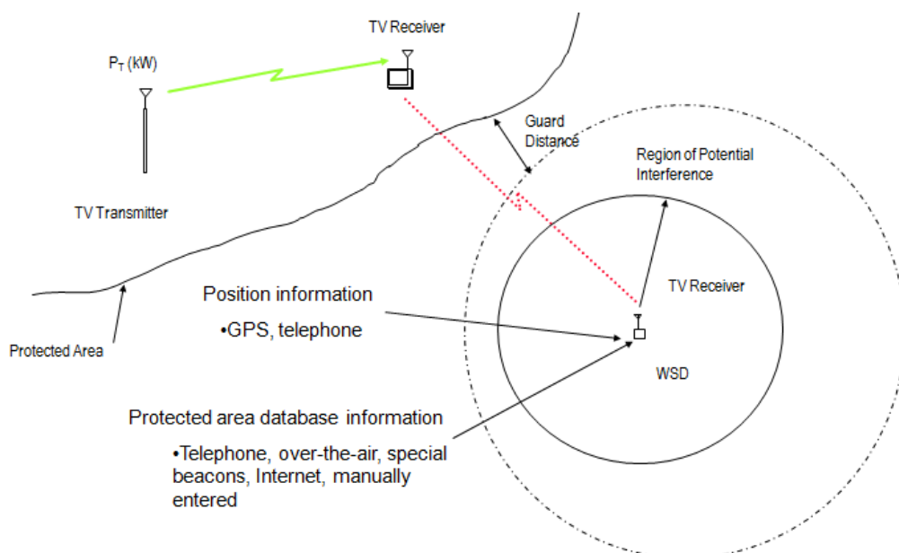
Figure 22 - General understanding of geo-location method.
