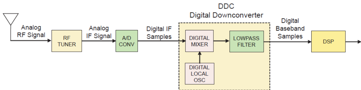
Figure 4 - SDR Receiver Block Diagram.
