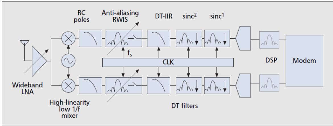
Figure 7 - Proposed SDR architecture.
