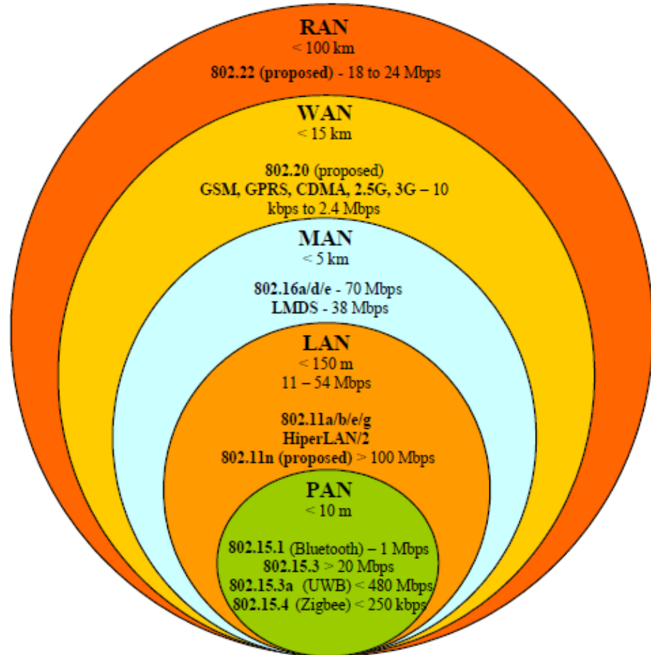
Figure 24. The IEEE 802.22 standard relative to other IEEE 802 wireless data transmission standards.
