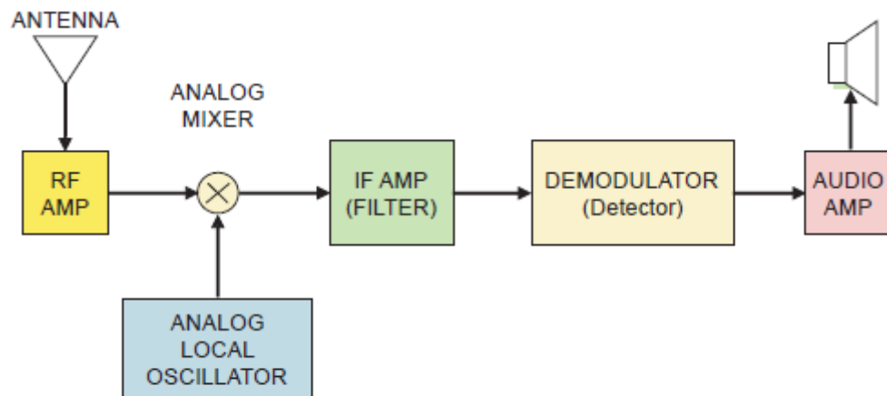
Figure 2 - Analog Radio Receiver Block Diagram.
