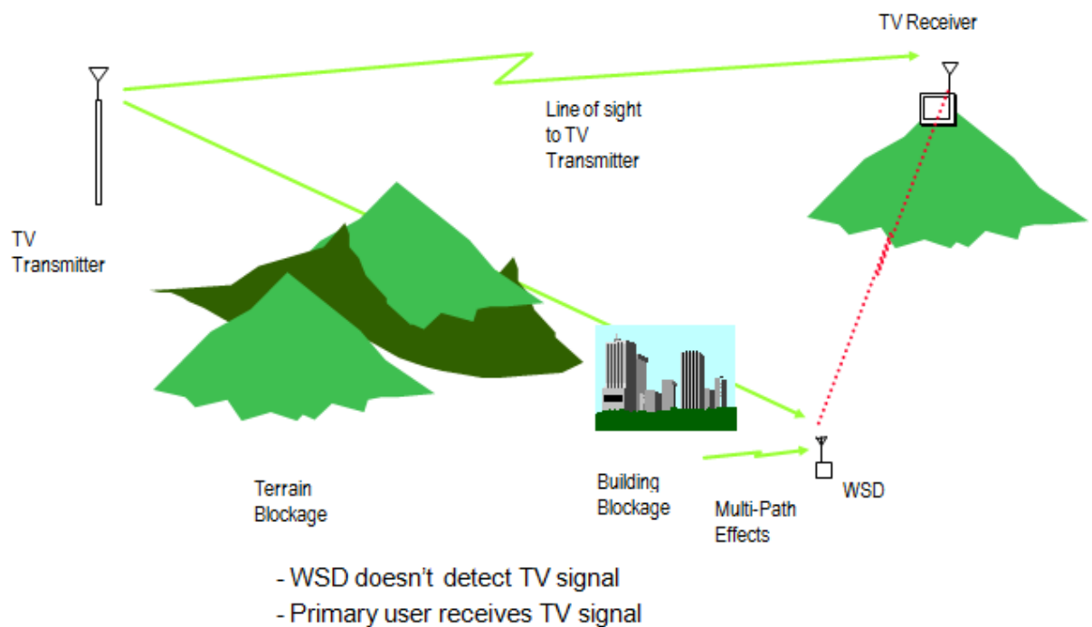
Figure 19 - Understanding of hidden node problem.
