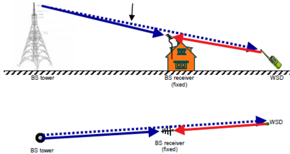
Figure 26 - Interference scenario example.
