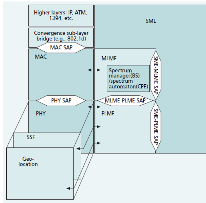
Figure 25 - The IEEE 802.22 reference architecture.
