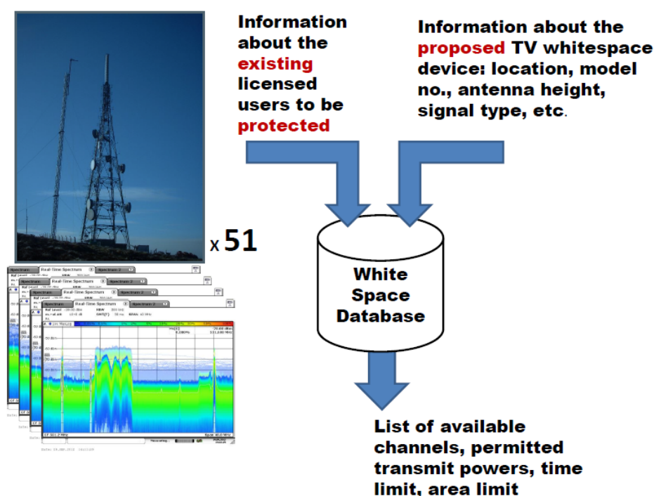
Figure 20 - Analysis of information of existing services to be protected and WSD location in order to create a list of available channels and permitted parameters on a Database.
