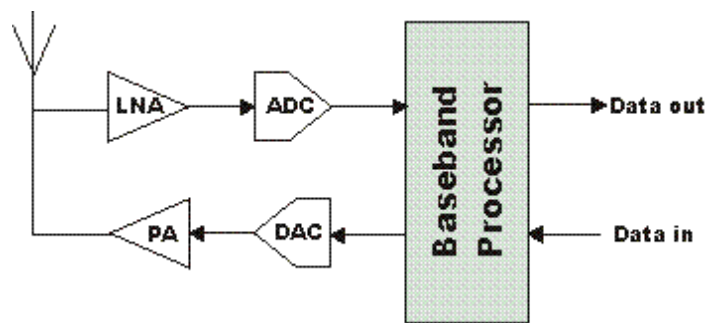
Figure 1 - Block diagram of an 'Ideal' Software Defined Radio
