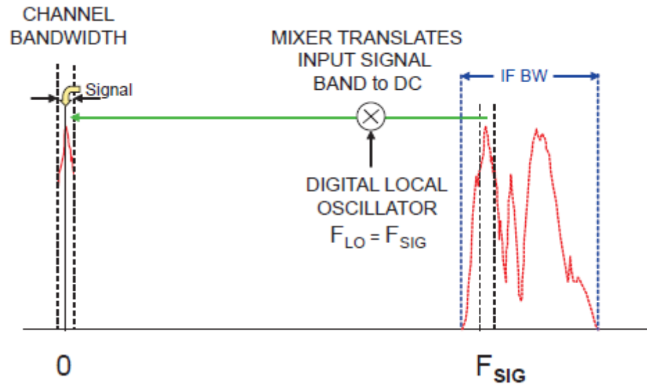
Figure 5 - SDR Receiver Mixer.
