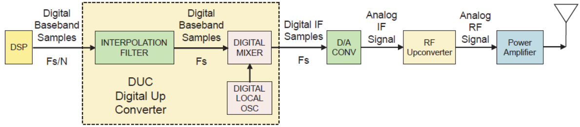
Figure 6 - SDR Transmitter Block Diagram.
