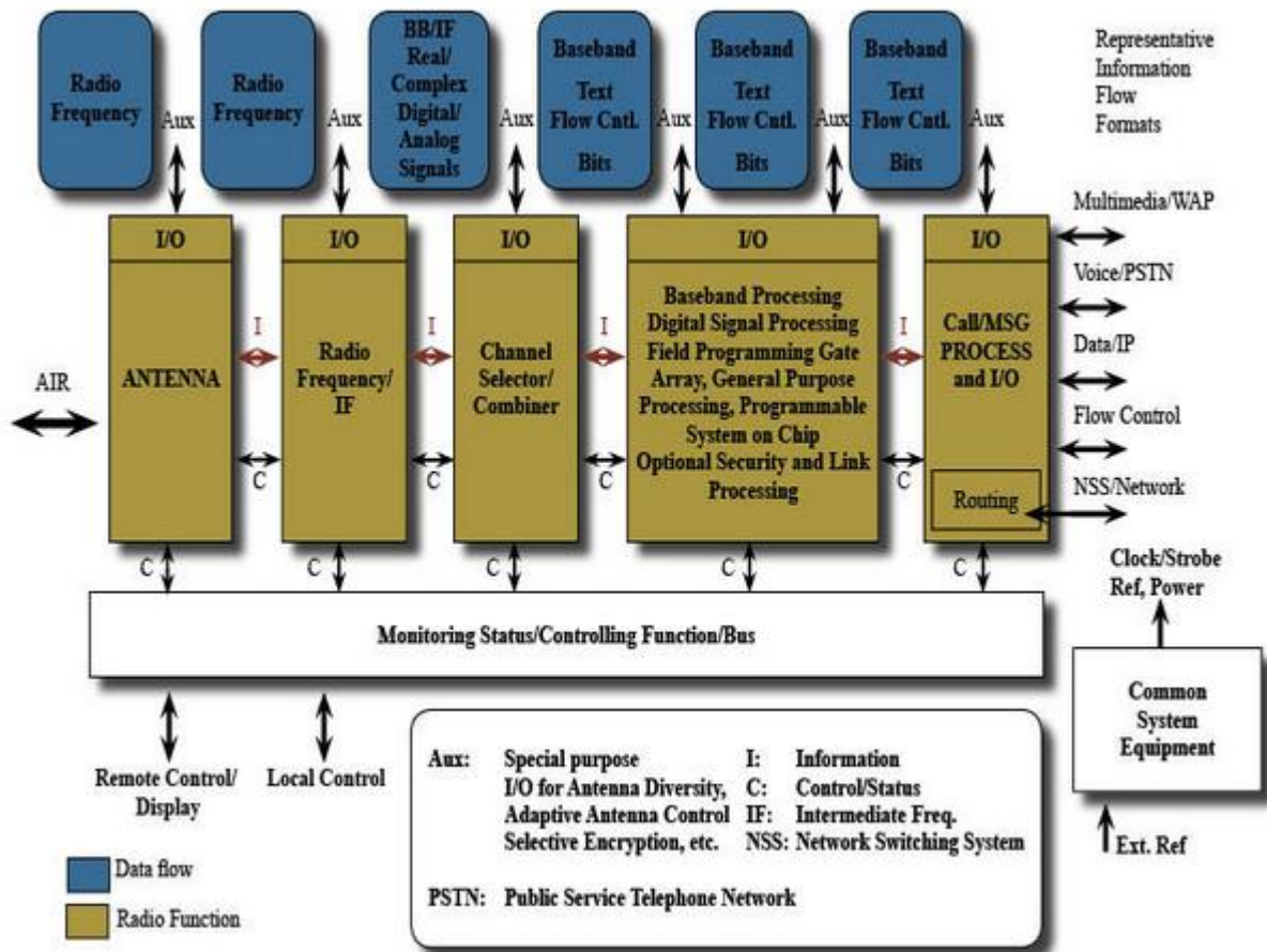
Figure 8 - Generalized Functional Architecture of SDR (Standardized Hardware Architecture by SDR Forum [7]).
