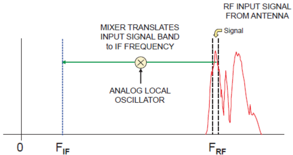
Figure 3 - Analog Radio Receiver Mixer.
