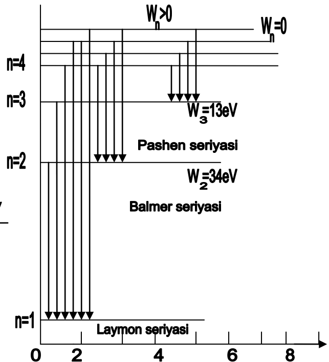
3-rasm Vodorod atomi energetik sathlarining diagrammasi
