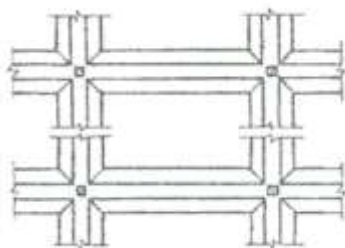
6.4- rasm. Jo'yaksim chorrha poydevor. 6.5- rasm. Yaxlit poydevor.
