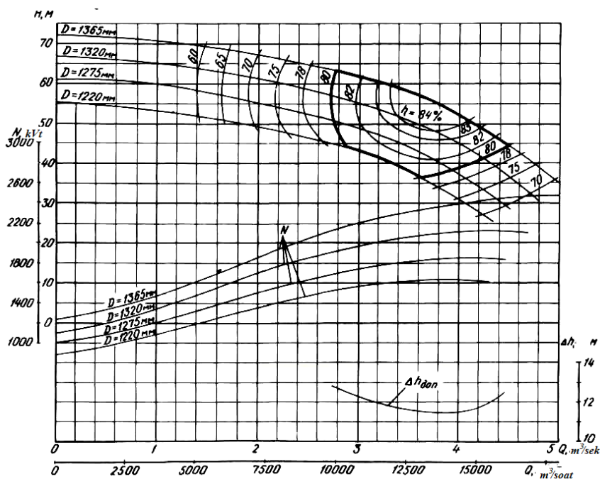
4.19-rasm. Vertikal markazdan qochma 1000V – 4/53 markali nasosning universal xarakteristikasi ( \Delta h_{dop} – kavitasiya zaxirasi chizig'i.)
