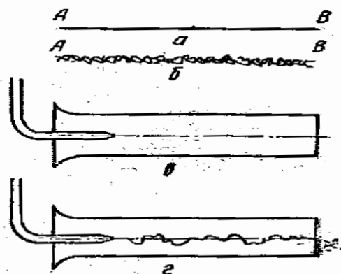
1.14-rasm. Turbulent va laminar harakatga doir chizma.
