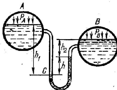
1.7-rasm. Differensial manometr.
