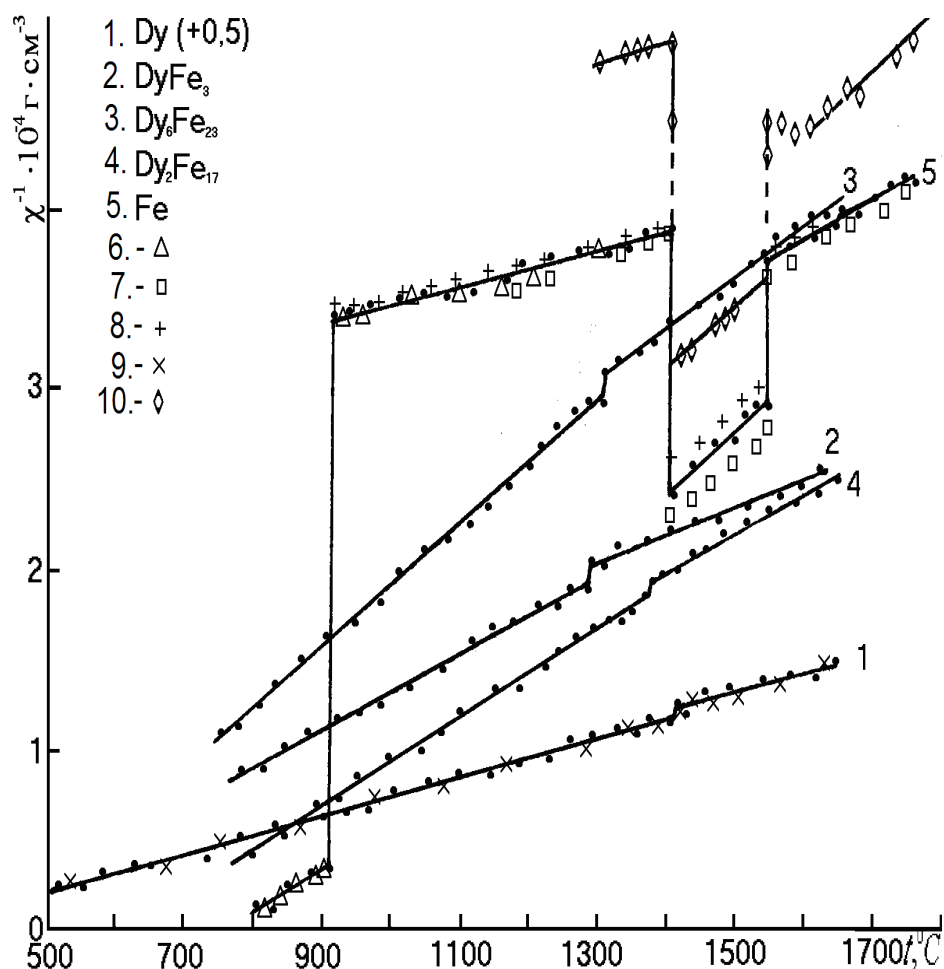
1.7-rasm.Dy-Fe
