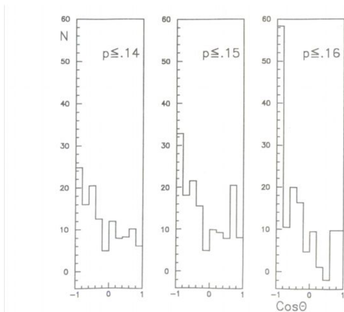
15-rasm. Tushuvchi uglerod yadrosining tinch holat sistemasida proton- spektatorlarning ularning impulsaridan bog'liq holdagi burchak taqsimoti (impulsar 0-0,14, 0-0,15, 0-0,16 GeV/c).
