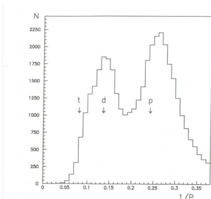
10-rasm. Zarrachalarning impulsning teskari qiymati bo'yicha taqsimoti ( 4 gradusdan kichik burchakda).
