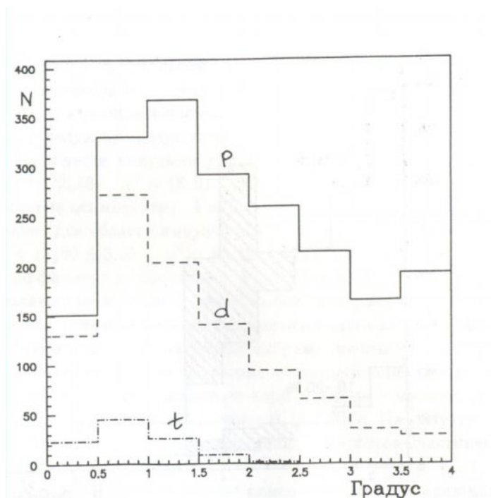
13-rasm. 0-4 gradus intervalida spektator zarrachalarning burchak taqsimoti.
