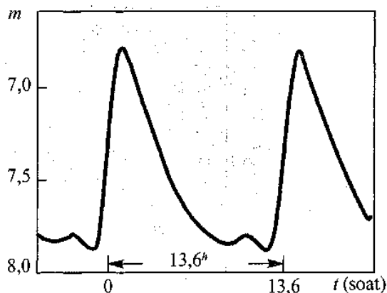
Rasm 5. Liraning RR o'zgaruvchi yuldizi ravshanligining o'zgarishi.
