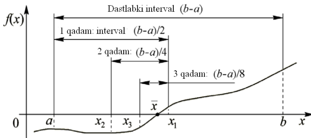
2.1–rasm. Kesmani ikkiga bo'lish usulining sxematik tasviri.
