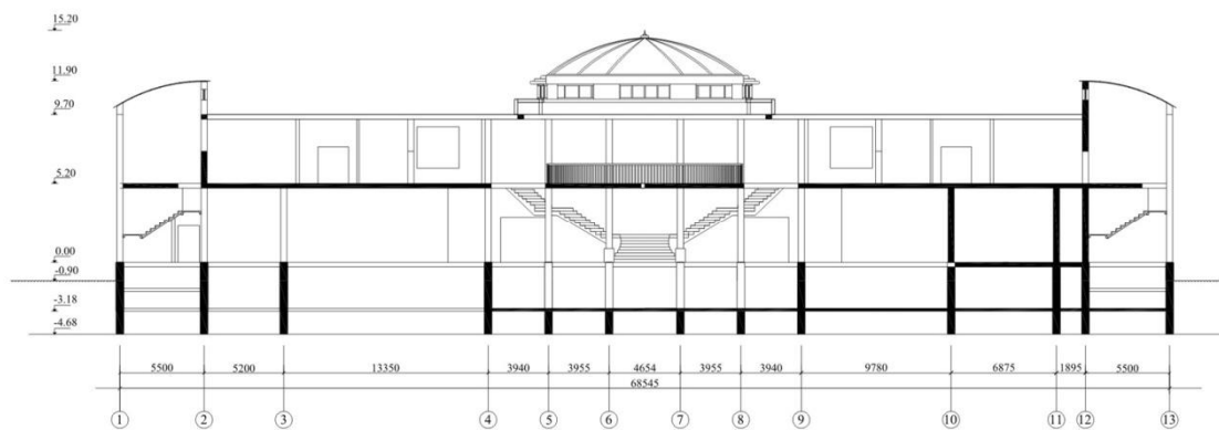
Qirqim 1-1 M 1:100
