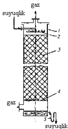
25.5-rasm. Nasadkali absorber:
