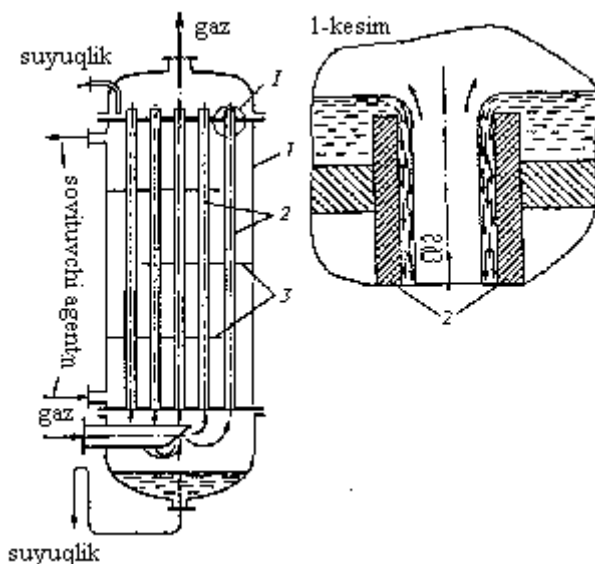
25.4-rasm. Quvurli plyonkali absorber: 1 — qobiq; 2 — quvurlar;
