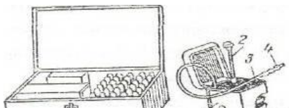
8.2.-rasm. UG-2 gaz tahlil qilgichi: 1-korpus; 2-so'rish quvuri; 3-indikator quvuri; 4-filtirlovchi patron; 5-silfon quvuri; 6-ampulali yashik.
