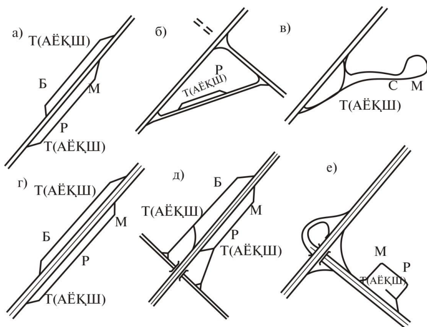
71-rasm. Yo'llarda harakatga xizmat ko'rsatish majmualari va korxonalarni rejalashtirishni printsiptial sxemalari (a-e):
