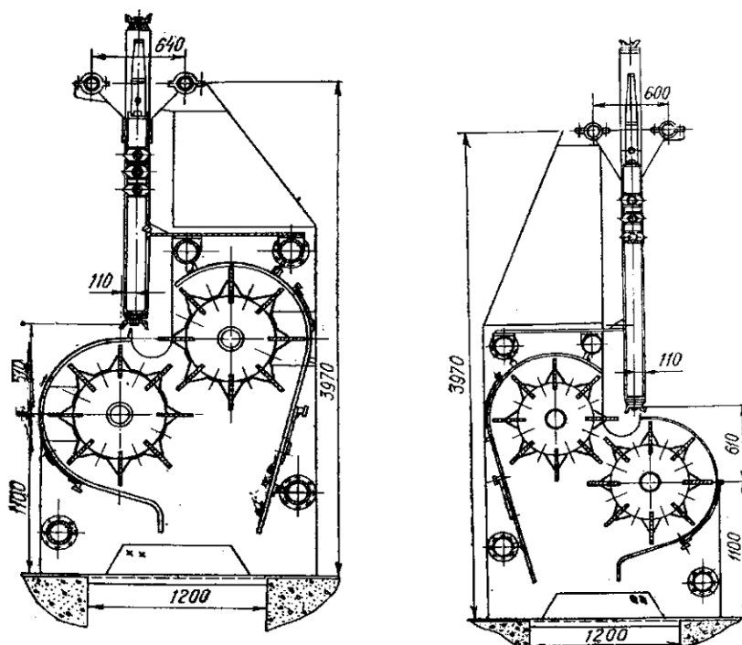
1-Rasm. AJIT rusumli titish-yuvish mashinasi
