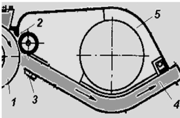
8.7-rasm. Tolani arra tishlaridan ajratuvchi moslamalar sxemasi
