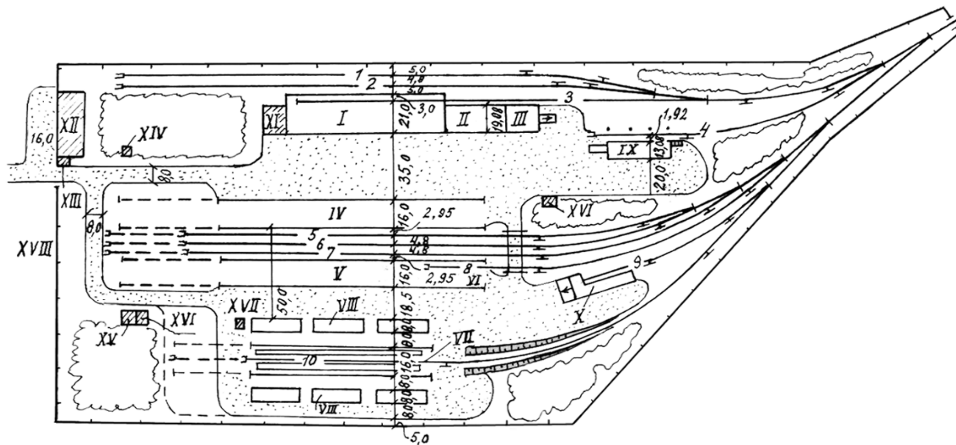
8-rasm. Boshi berk yo`lakli tipdagi yuk hududi sxemasi:
