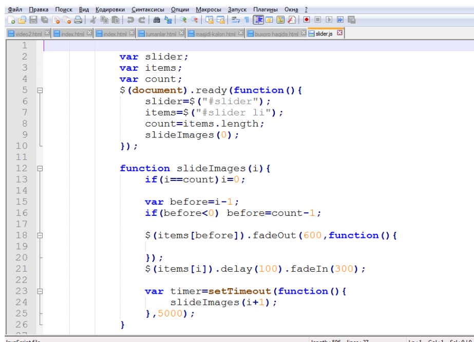
13-rasm. Slyder JavaScript tarkibi
