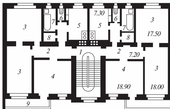
4-rasm. Turar joy loyihasi:
