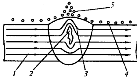
3 - rasm. Magnit-kukunli usul chizmasi:
