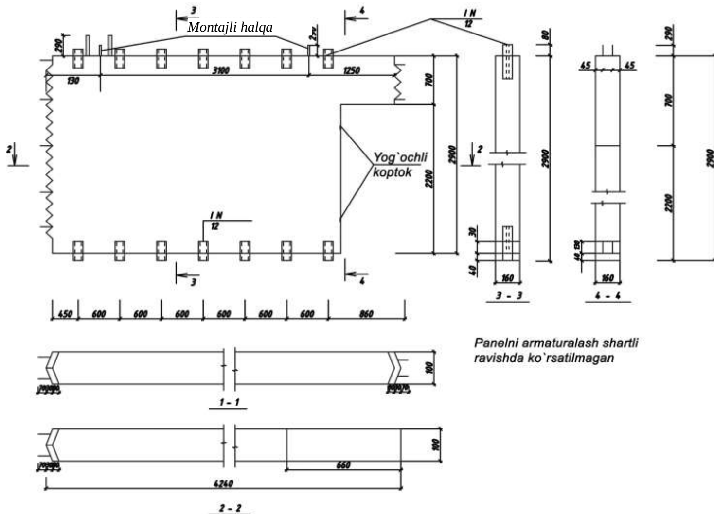
4.5-rasm. Ichki panel devori.
