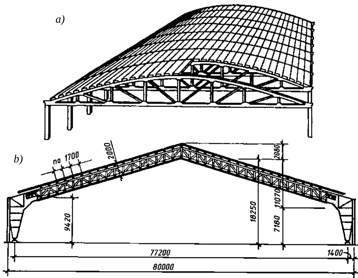
7.41-rasm. Katta oraliqli silliq tom.
