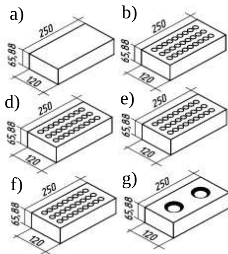
2.21-rasm. Sopol g‘isht:
