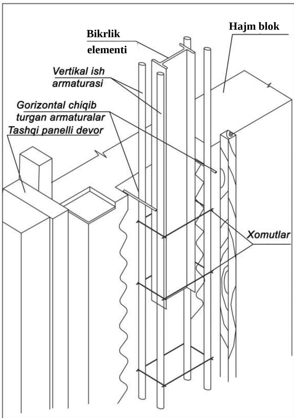
5.11-rasm. I-tugun /aksonometriya/.
