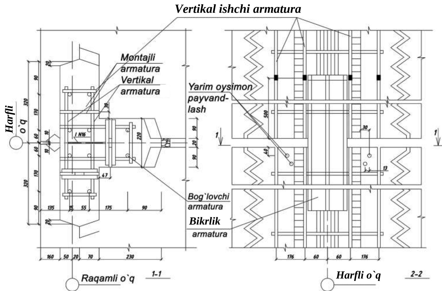
5.14-rasm. 4-tugun.
