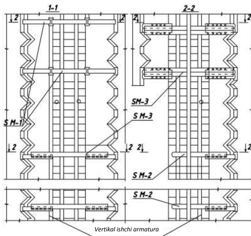
Qirqim 1-1; 2-2.
