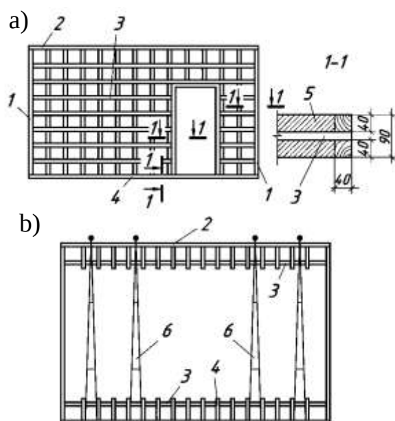
2.55-rasm. Parda devor paneli yog‘och karkasining sxemasi:
