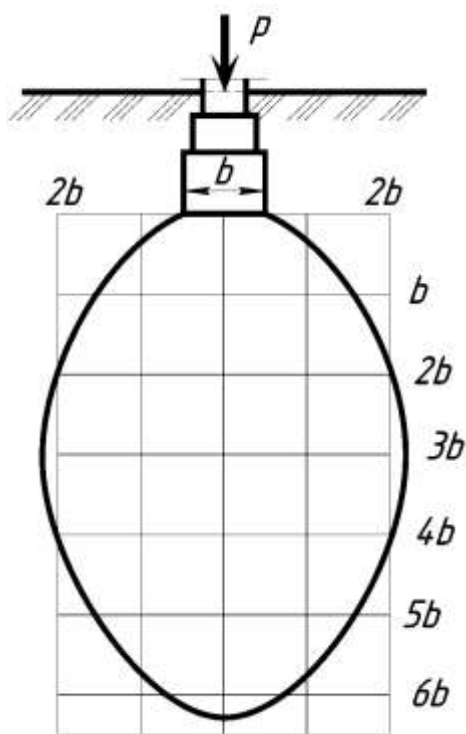
2.7-rasm. Poydevor osti zamin gruntida yuzaga keladigan zo'riqish zonasi:
