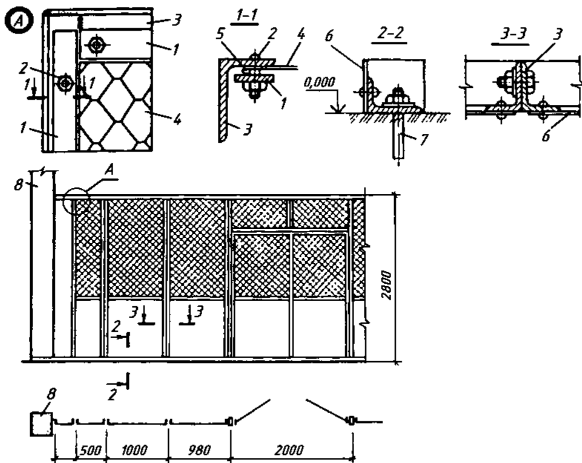
7.58-rasm. Metall to'rli devor:
