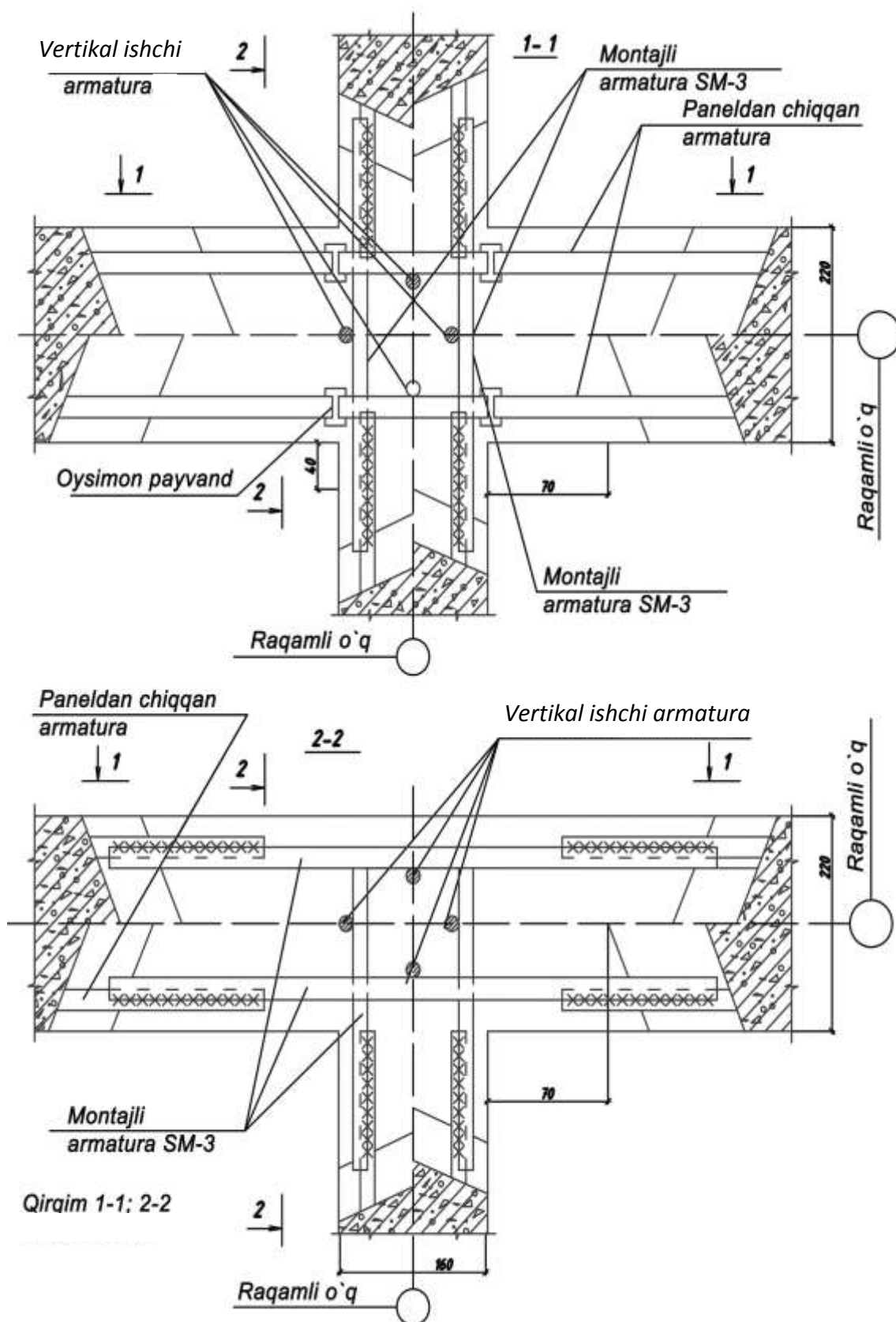
4.9-rasm. Ichki panelli devorlarning tutashishi. Qirqim 1-1; 2-2.
