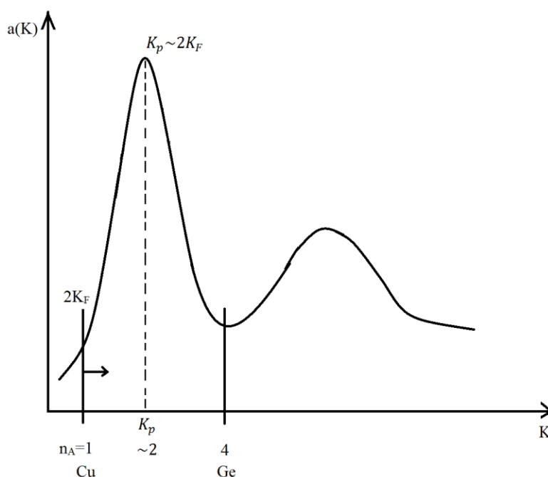
3.2.6 – rasm.Kopvalentli metal qotishmalar uchun interfirinsion funksiyaning ko' rinishi.
