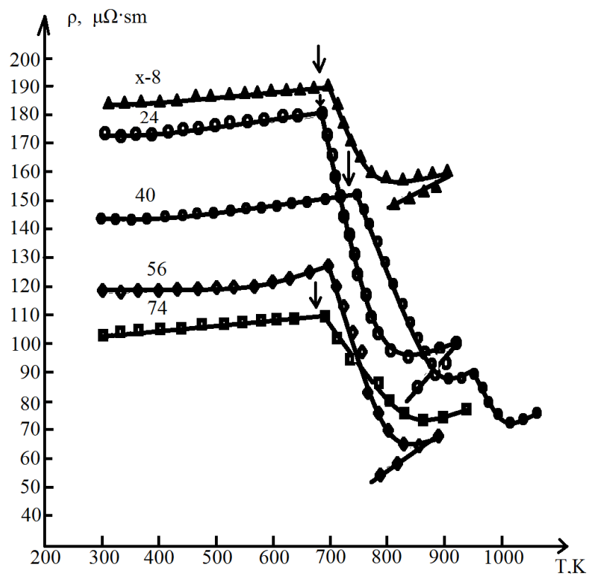
3.4.2-rasm. \text{Fe}_{80-x}\text{Co}_x\text{B}_{20} sistemasining solishtirma elektr qarshiligining temperaturadan bog'liqligi
