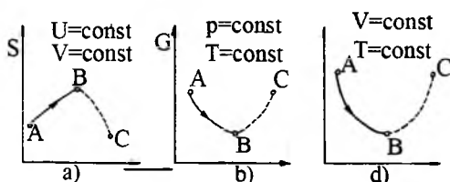
12-rasm Turli jarayonlarda entropiyaning o‘zgarishini ifodalanishi
