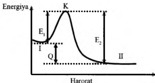
35-rasm. Reaksiyada energiyani o'zgarishi.
