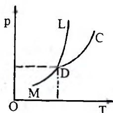
29-rasm. Erish (kristallanish) haroratining bosimga bo‘liqligi.
