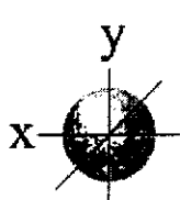
S – orbital
