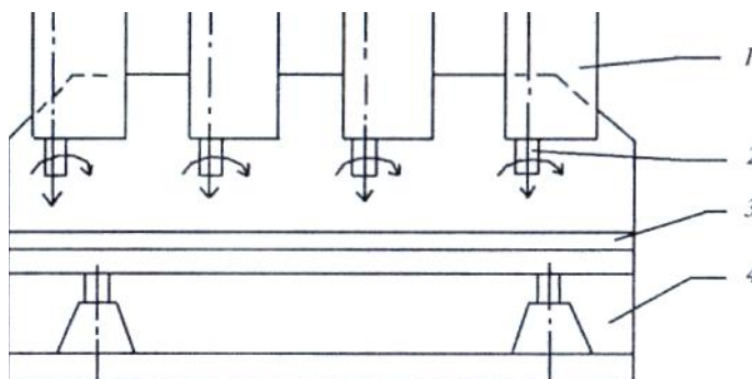
8.3-rasm. To'rt shpindelli vertikal-parmalash stanogi:
