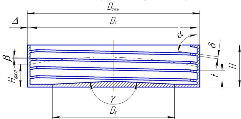
1-rasm. Titrama yuklovchi qurilmaning ko‘rinishi
