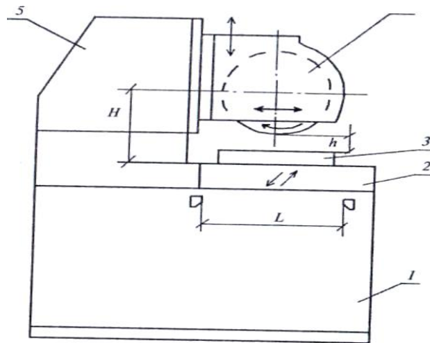
8.15-rasm. Yassi jilvirlash stanogi.
