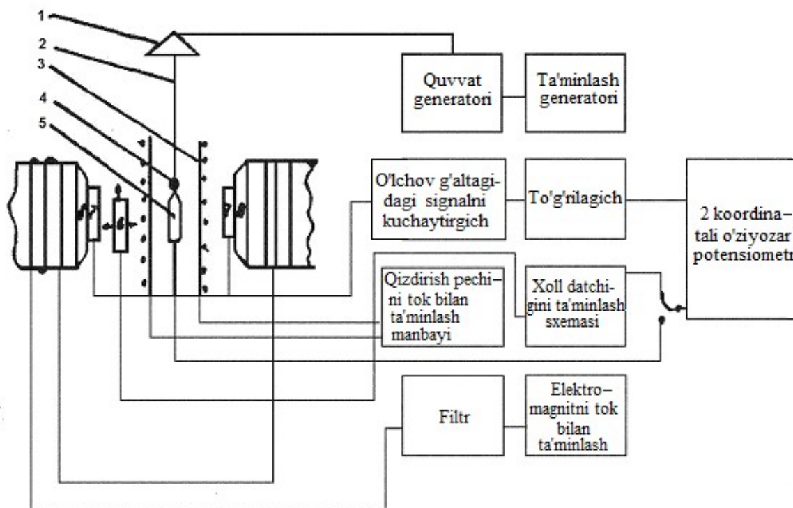
1-rasm. Magnitlanishni o'lchovchi tebranuvchi magnetometr qurilmasining sxemasi. 1-tebratgich, 2-sterjen, 3-elekr isitish pechi, 4-namuna solingan ampula, 5-termopara, 6-Xoll datchigi, 7-induktiv datchigi, 8- elektromagnit.
