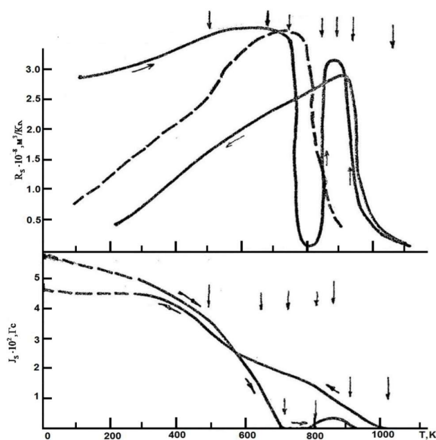
2 – rasm. Co_{84.35}Fe_{5.8}Si_{7.4}B_{2.45} qotishmaning Xoll koeffitsienti (yuqoridagi rasm) va magnetlanishi (pastki rasm) ni temperaturaga bog'liqligi.
