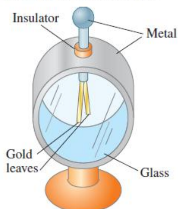
FIGURE 16-10 Electroscope.
