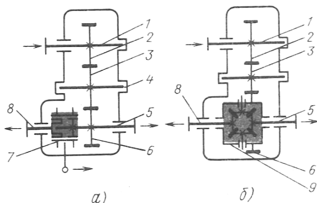
12.3-rasm. Taqsimlash qutilarining sxemalari:
