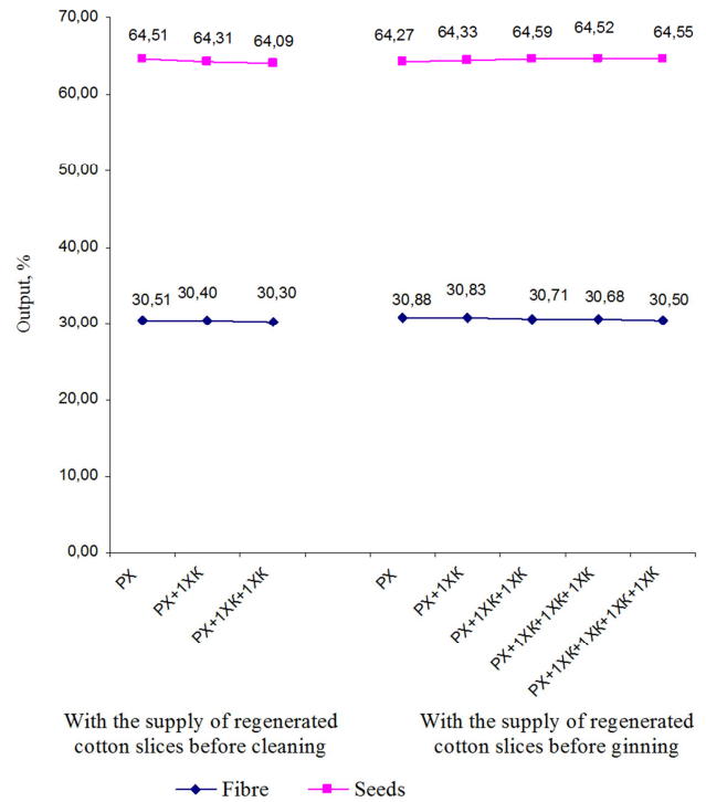
Figure 6. The output of fiber and seeds, depending on the purifying plan and places for feeding raw regenerated bales.
