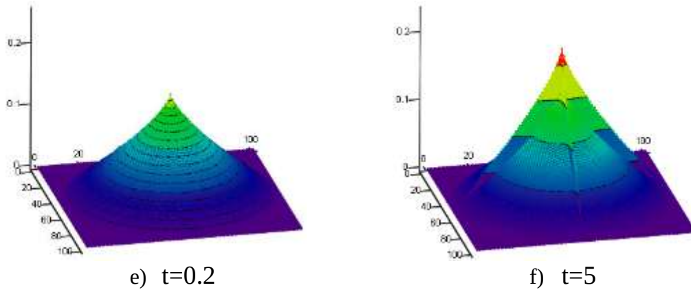
Fig 3. Numerical solution of the problem (17)-(19): p=3, q=3, l=1,5, m=0.5, n=2.(q=l(p-1)) .
