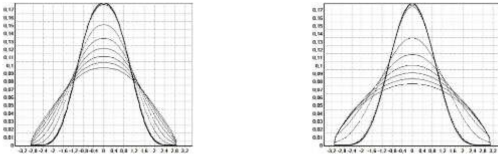
Fig 4. Numerical solution of the problem (17)-(19) when m=1.5 , p=1.75 , q=2.85 , 1) n=0 , 2) n=-0.25 .
