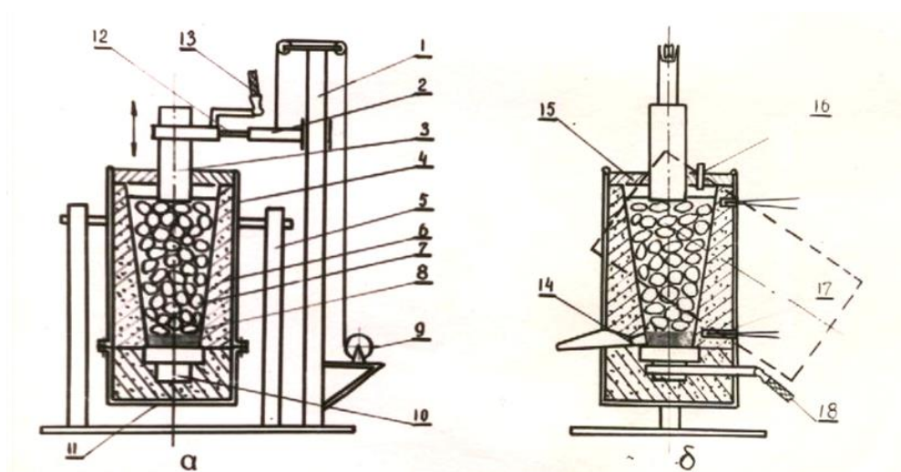
Figure 1. Installation for remelting aluminum scrap
